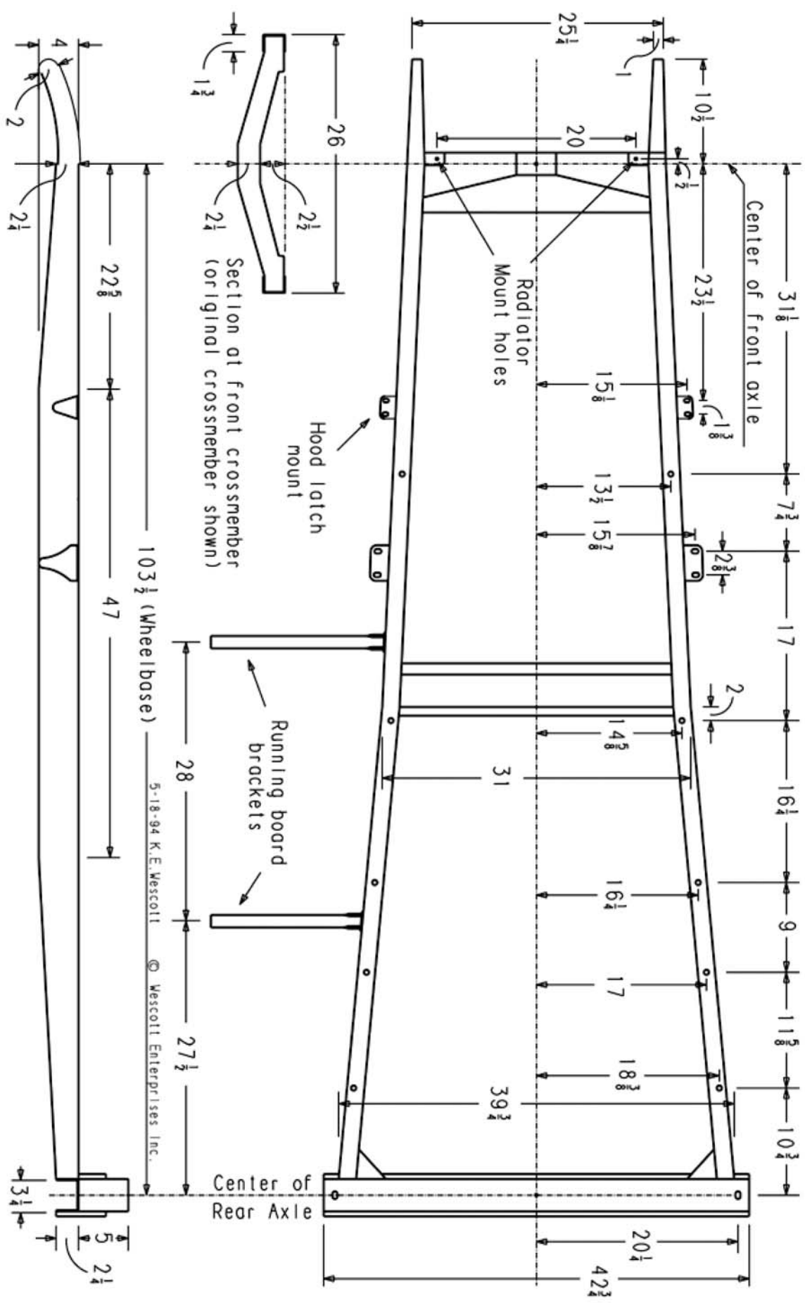
1928-31 Ford Model "A" Frame diagram only measurements in inches Passenger cars and Pickups use same frame
