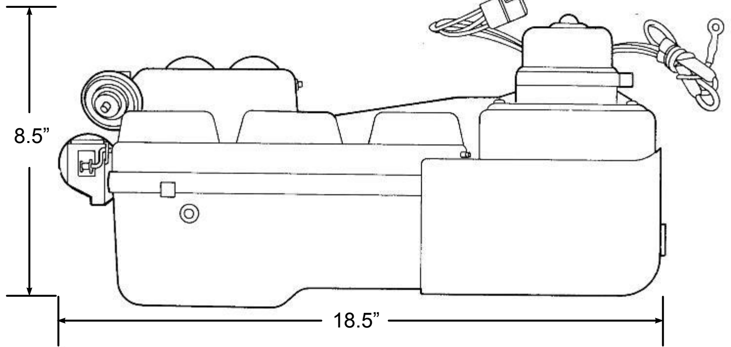
Front View
